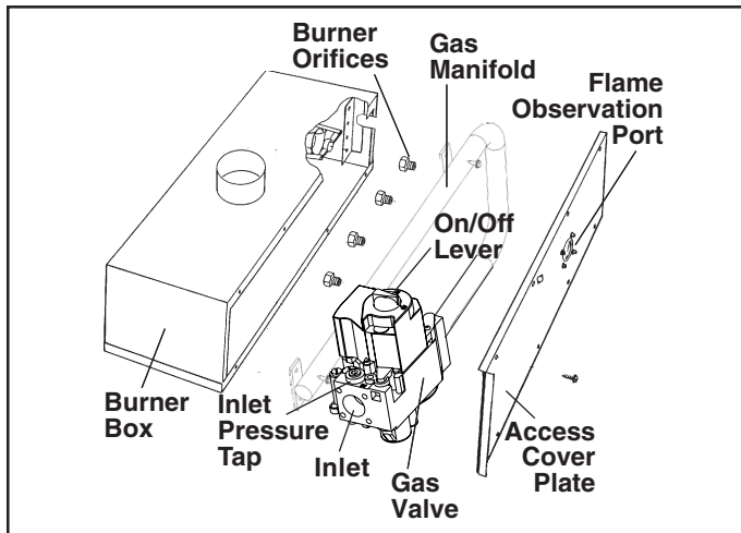
Figure 2. Typical Sealed Burner Box With Access Cover Plate
