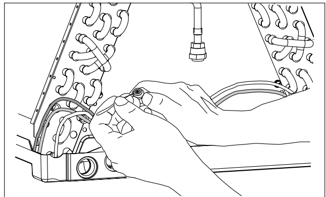
Figure 5. Restrictor Insertion in Distributor Body
