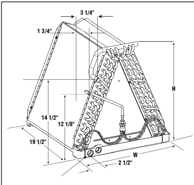
Figure 1. B & C Cabinet Coil
